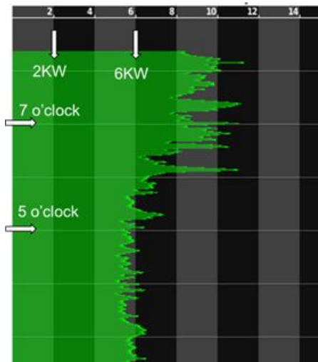
Fig. 7 Electric Demand of 20 Houses
