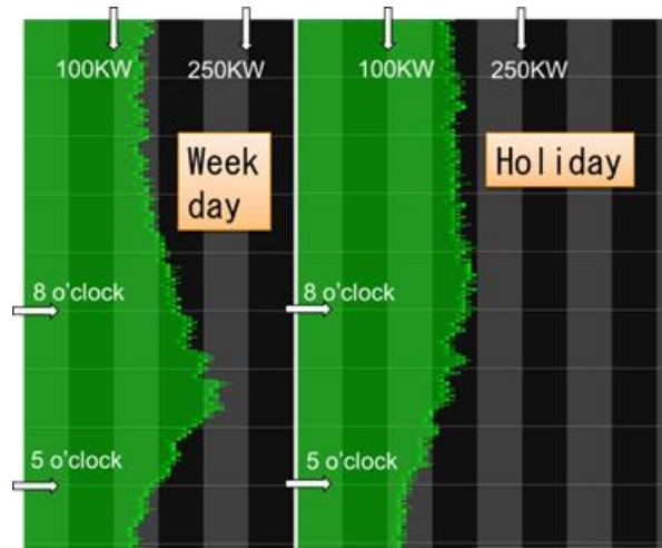
Fig. 8 Electric Demand of 309 Houses
