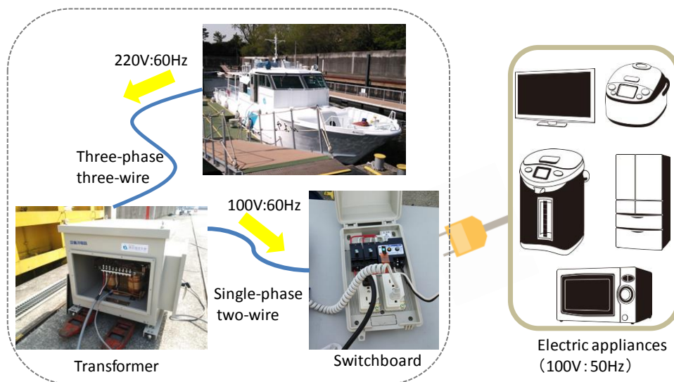
Fig. 9 Ship-to-Land, power supply system at emergency
