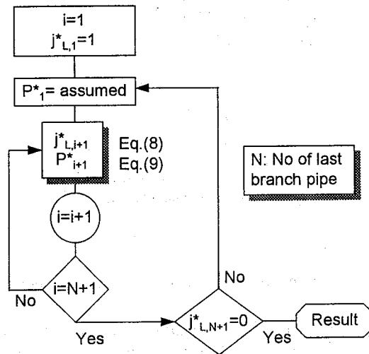
Fig. 3. Iteration procedure.
