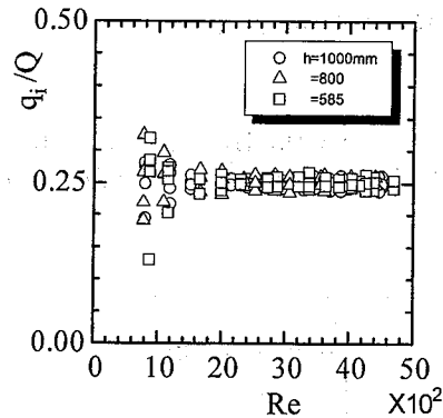
Fig. 7. Flow distribution for single-phase fluid.
