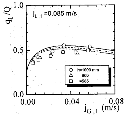
Fig. 13. Water flow rate to first pipe at j_{L,1} = 0.085 m/s.
